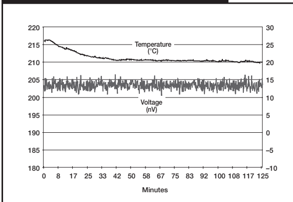
The Model 2182 measuring a 10mΩ resistor with a 20μA test current on the 10mV range using the Delta mode.
