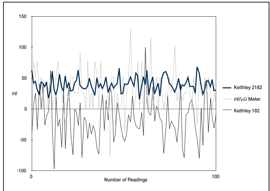
This graph compares the Model 2182's noise performance with that of the Model 182 and a Nanovolt/Micro-ohmmeter. All the data shown was taken at 10 readings per second with a low thermal short applied to the input.
